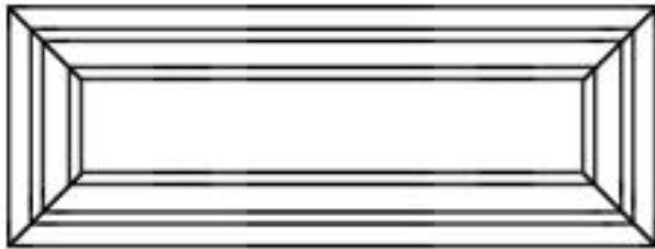
1051 MR-1 DF Square Mitered Reversed Raised Panel Minimum Width: 7 1/2" Minimum Height: 6 1/2"
