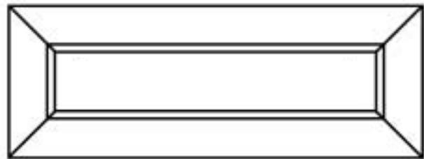
1053 MR-3 DF Square Mitered Reversed Raised Panel Minimum Width: 7 1/2" Minimum Height: 6 1/2"
