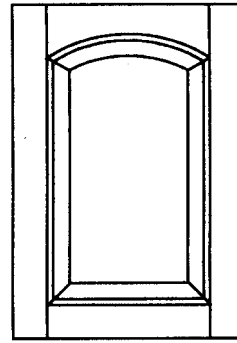
104 Eyebrow Raised Panel Minimum Width: 7 1/2" Minimum Height: 10"
