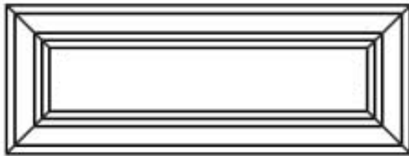
1053 MR-3 DF Square Mitered Reversed Raised Panel Minimum Width: 7 1/2" Minimum Height: 6 1/2"
