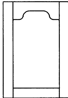
808 Flattop Reversed Raised Panel Minimum Width: 9 3/4" Minimum Height: 10"
