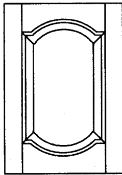
107 Double Shoulder Eyebrow Raised Panel Minimum Width: 9 3/4" Minimum Height: 12"
