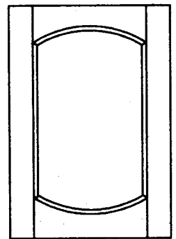
205 Double Eyebrow Flat Panel Minimum Width: 7 1/2" Minimum Height: 11"
