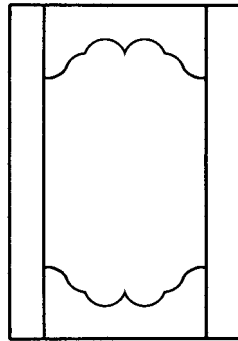
813 Double Clover Reversed Raised Panel Minimum Width: 14" Minimum Height: 13"
