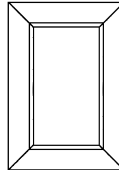
1004 MR-4 Squared Mitered Reversed Raised Panel Minimum Width: 9" Minimum Height: 9"
