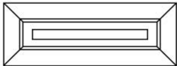
554 MR-4 DF Square Mitered Raised Panel Minimum Width: 7 1/2" Minimum Height: 6 1/2"
