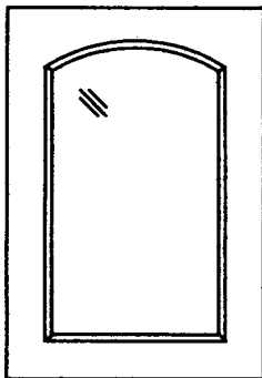
404GL MDF Eyebrow Glass Panel Minimum Width: 8" Minimum Height: 10"
