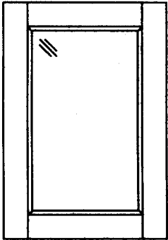
601GL Square Glass Panel Minimum Width: 7 1/2" Minimum Height: 7 1/2"
