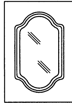
303GL-MDF Double Cathedral Raised Panel Minimum Width: 10 13/16" Minimum Height: 12"
