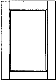
201 Square Flat Panel Minimum Width: 7 1/2" Minimum Height: 7 1/2"
