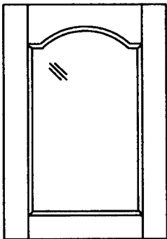
606GL Shoulder Eyebrow Glass Panel Minimum Width: 7 1/2" Minimum Height: 9"
