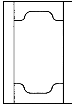
809 Double Flattop Reversed Raised Panel Minimum Width: 9 3/4" Minimum Height: 12"
