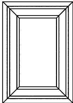
703 MR-3 Mitered Flat Panel Minimum Width: 7 1/2" Minimum Height: 7 1/2"
