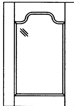
608GL Flattop Glass Panel Minimum Width: 9 3/4" Minimum Height: 10"
