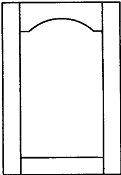
806 Shoulder Eyebrow Reversed Raised Panel Minimum Width: 7 1/2" Minimum Height: 9"
