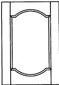
207 Double Shoulder Eyebrow Flat Panel Minimum Width: 7 1/2" Minimum Height: 12"
