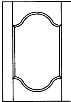
203 Double Cathedral Flat Panel Minimum Width: 7 1/2" Minimum Height: 12"
